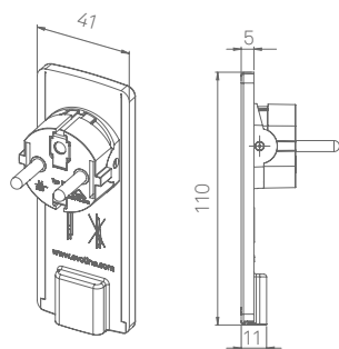
Plug Fix
